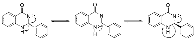
Figure 3. Proposed mechanism of racemization for compound 6 .
