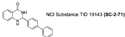
Figure 1. Structure of 2-biphenyl-2,3-dihydroquinazolinone.
